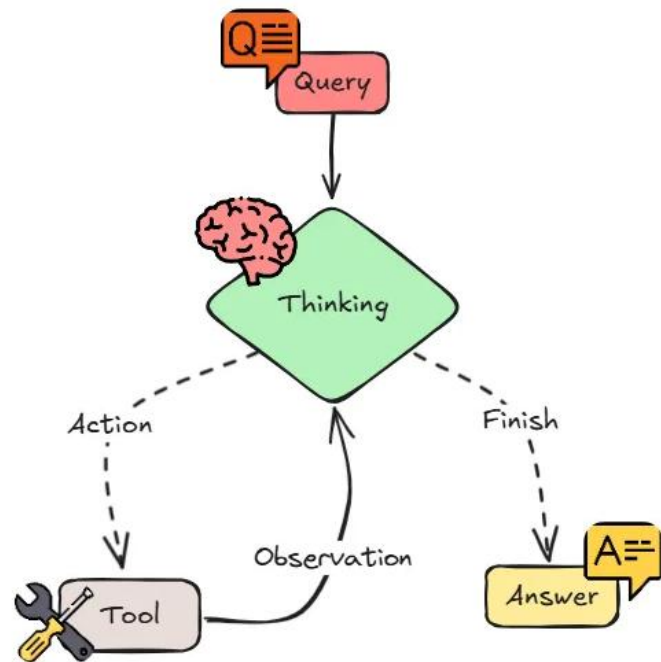
ReAct Agent architecture
